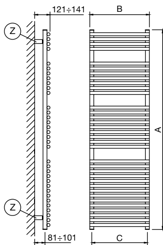
Mod. HG23150...
