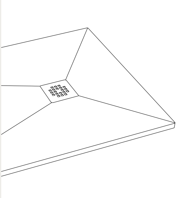
Installazione in appoggio Shower tray installation floor-mounted
