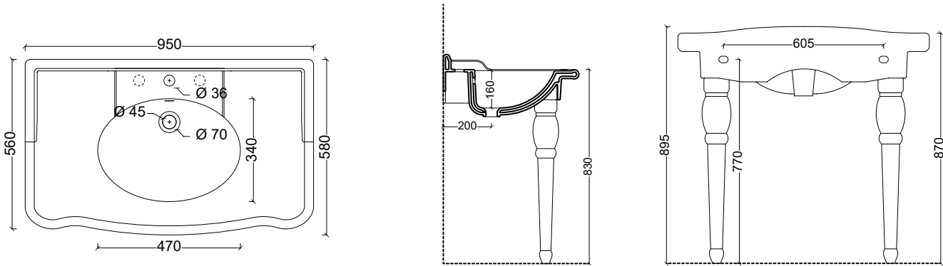
28260101 Lavabo Consolle BOHEME 95
