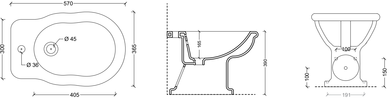
28220101 Bidet a terra BOHEME
