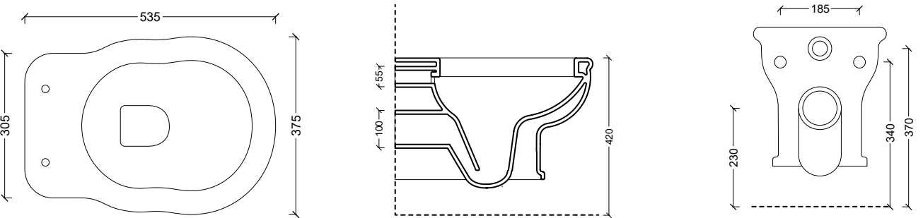
28230101S Vaso sospeso BOHEME
